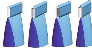
ALUMINUM TUBE FOLDING PATTERNS
